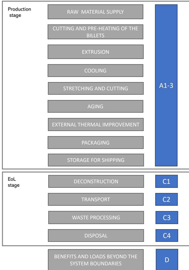
Figure 1. Scheme of the profiles manufacturing process occurring in Montreal
